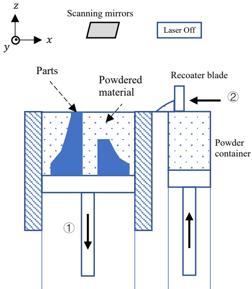
Powdered material layering
